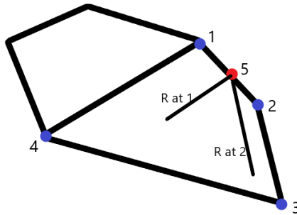
Fig. 3 Adjacent factors for polygons
