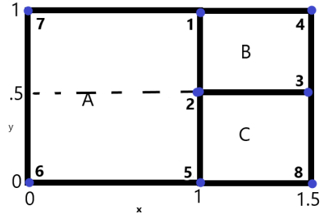
Fig. 2 Example of Incompatible Elements
