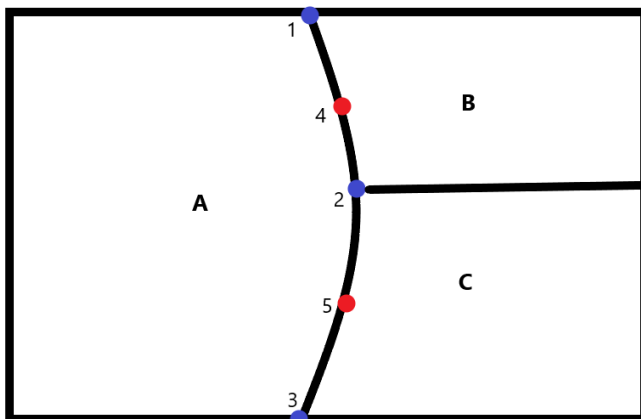
Fig. 7 Compatible quadratic variation on a parabolic side
