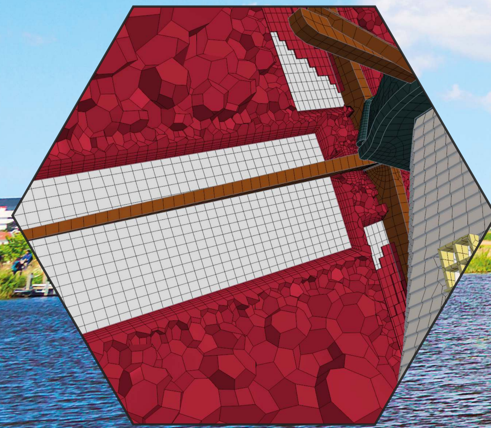
Polyhedra and prism layers from a quad surface mesh
