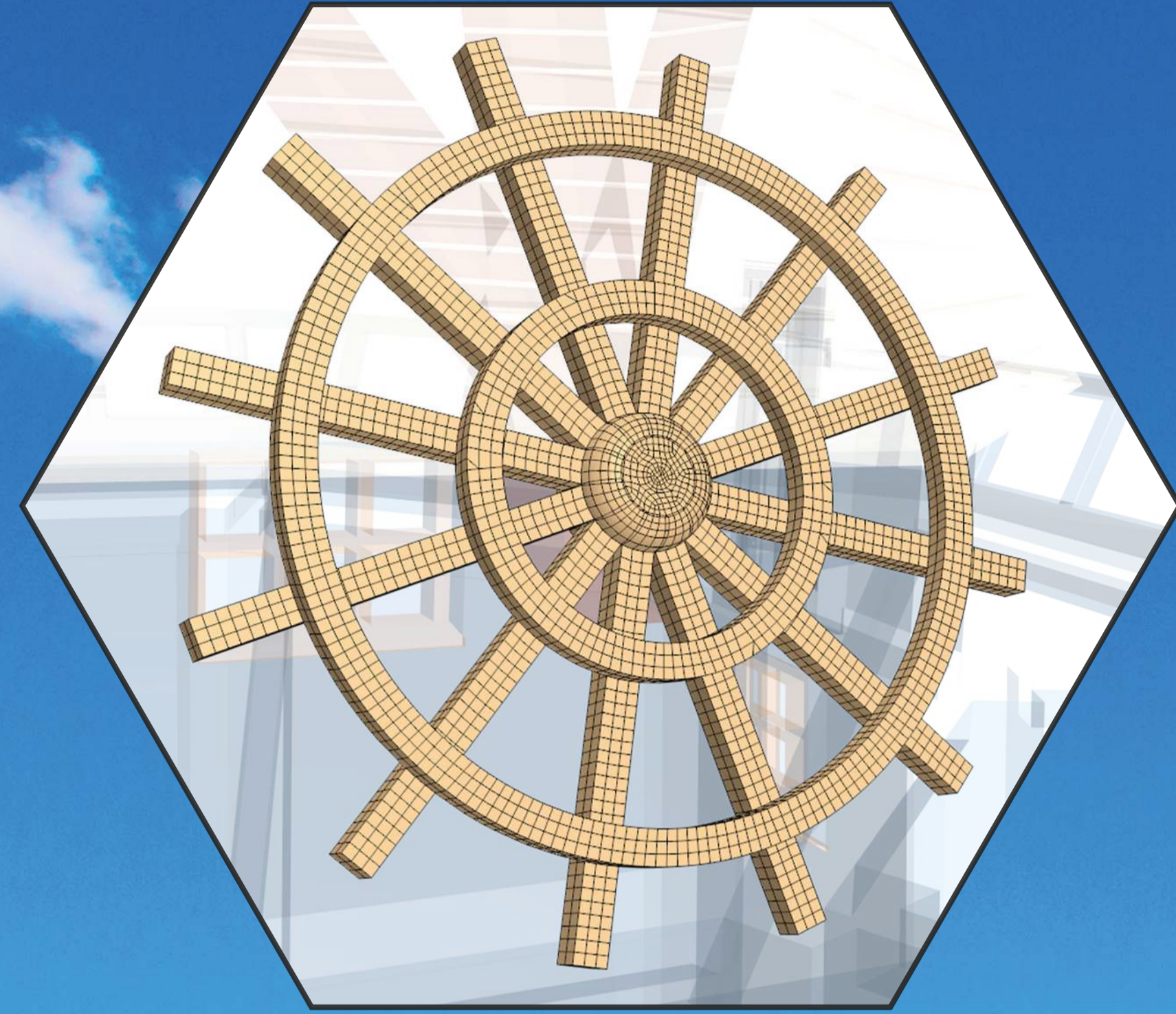
Swept mesh using multiple source and target surfaces
